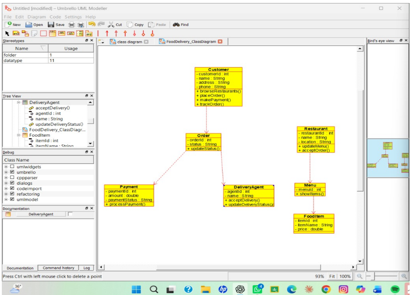
Figure 1: Class Diagram
